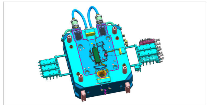
INVERTER HOUSING
